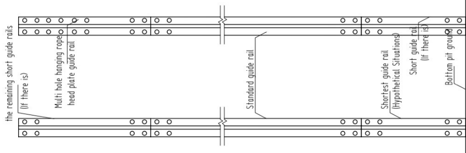
Schematic diagram of host side guide rail non host side guide rail
